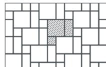
BOX PATTERN 2 1-6 x 6 (14%), 1-6 x 12 (29%), 1-12 x 12 (57%) 1-12 x 12 (14%), 1-12 x 24 (29%), 1-24 x 24 (57%)
