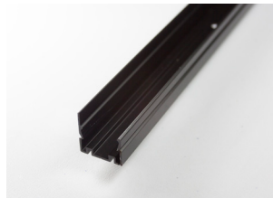
Strip Light Channel* (Gen 2) w/ Groove & Glare Shield Part Number: BRI-SL-A-C2 1M (3.2') Channel sections 5 - Screws
