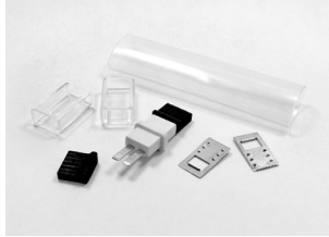
Double-Sided Connector Kit Part Number: BRI-SL-A-DSC 1 - Double-sided connector 2 - Clear plastic retainers 2 - Metal anti-slip plates 1 - Heat shrink tube
