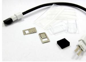
Jumper Connector Kit Part Number: BRI-SL-A-JC 1 - Jumper connector (10") 2 - Clear plastic retainers 2 - Metal anti-slip plates 2 - Heat-shrink tubes
