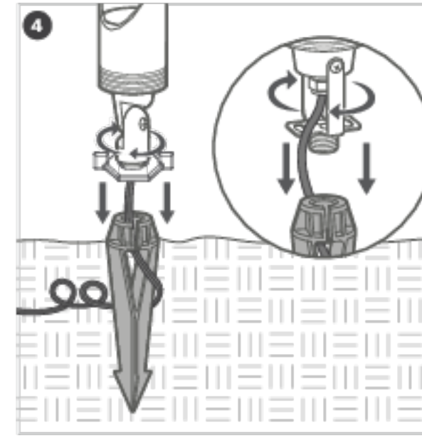
Wire Connections
