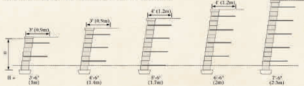
REINFORCED WALLS — Battered (9.5° +/- setback)
