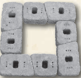
38" Pier, 1st and odd numbered courses
