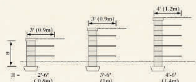
REINFORCED WALLS — Battered (9.5° +/- setback)
