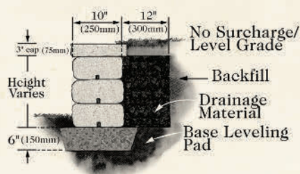
Gravity Wall – Near Vertical Detail
