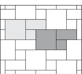
Random Pattern 1 24x24 (57%), 12x24 (29%), 12x12 (14%)
