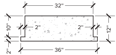
Grill Insert Concrete Filler Piece
