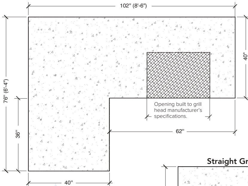
L-Shaped Grill Station Counter Top
