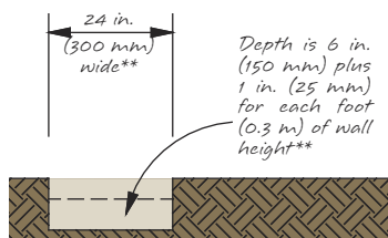
Excavate
