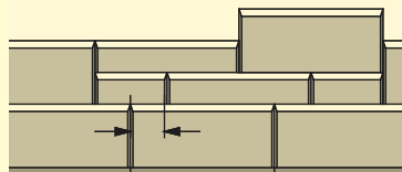
Offset by at least 1/4 of the block
