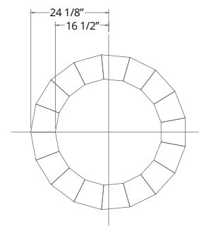
Laredo circle using Tapered Units 17 units required for full circle.
