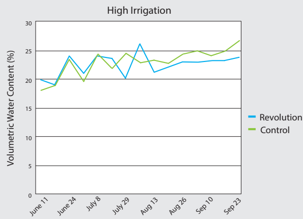
Figure 2. Revolution maintained similar VWC in plots irrigated at a high irrigation threshold of 16% VWC. (Dr. Kevin Frank, Michigan State, 2013)
