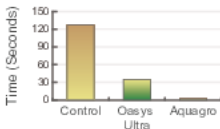
Sumitomo Chemical Co. Experimental Farm, Japan Water Infiltration Rate
