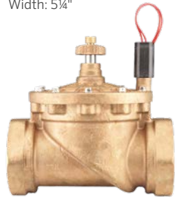
IBV-301G-FS Inlet diameter: 3" Height: 9" Length: 8½" Width: 7"
