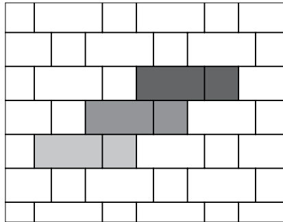
COURSED RUNNING BOND
