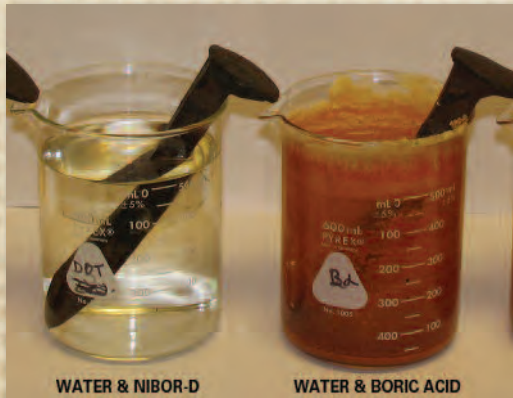
Nibor-D vs. Boric Acid Corrosion Comparison
